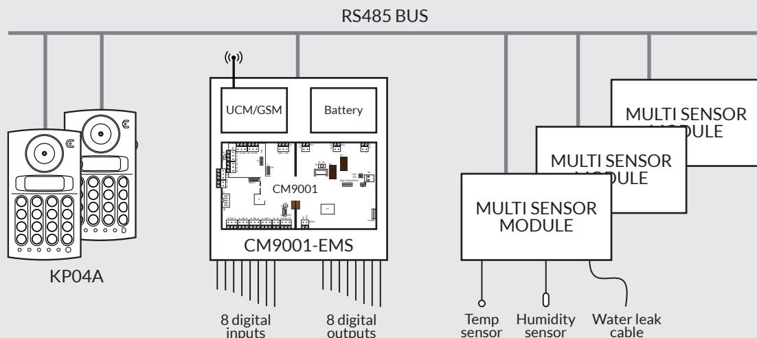
Schematic of CM9001-EMS with MSM01 Modules
