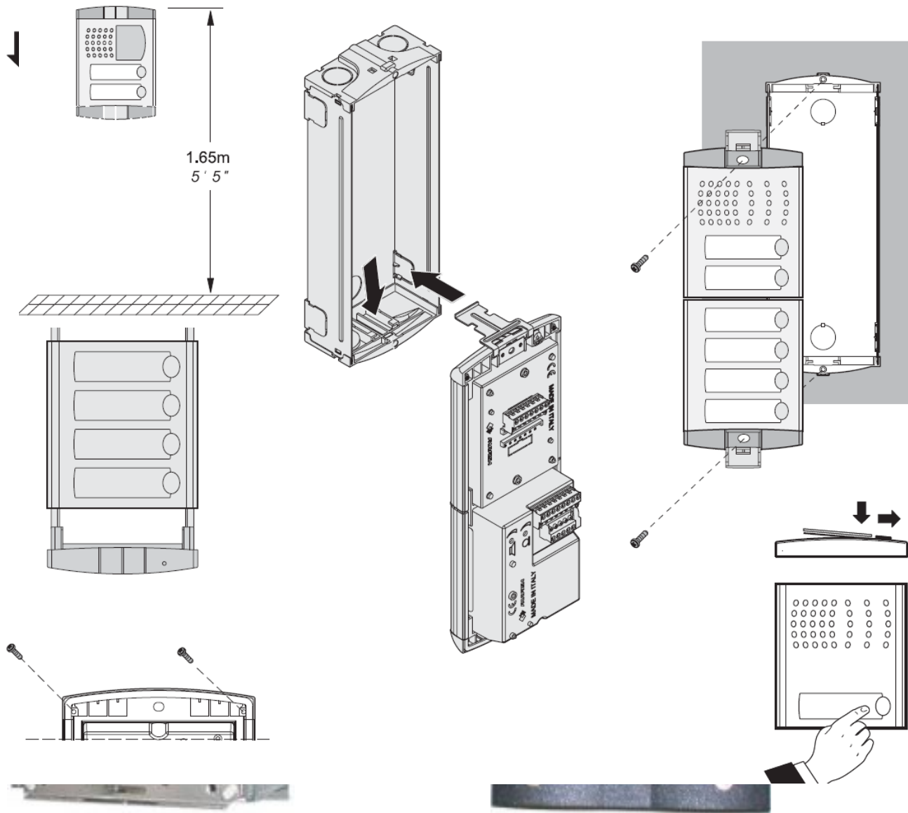
MA71 – Backbox for flush mount
